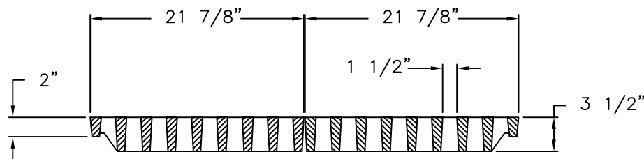
GRATE SECTION
