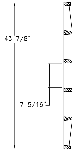
GRATE SECTION
