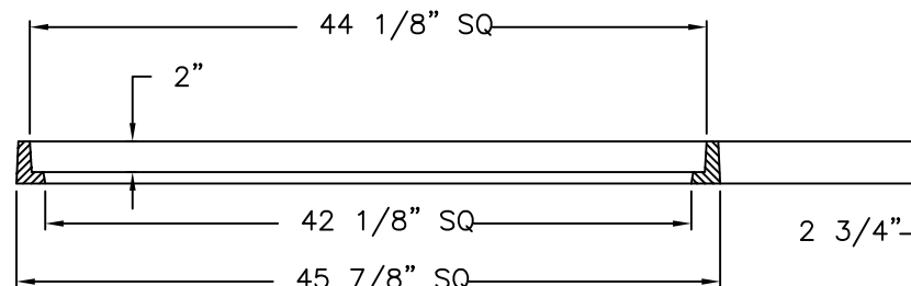
FRAME SECTION
